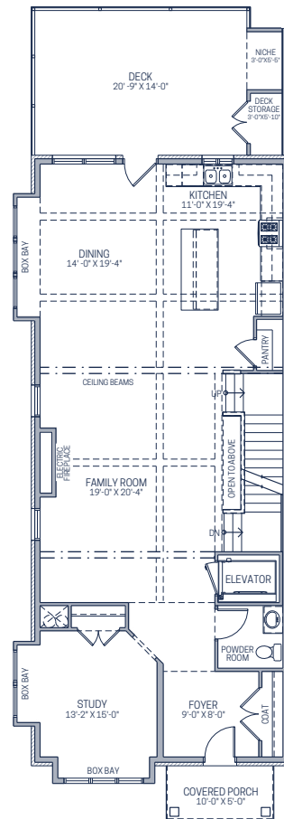
FIRST FLOOR PLAN LOT 108
