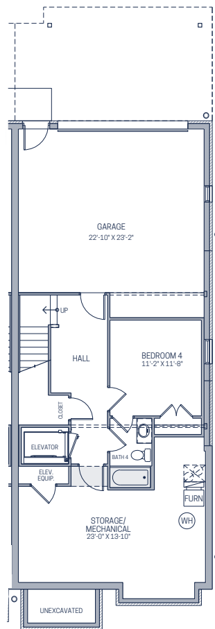
LOWER LEVEL PLAN LOT 110
