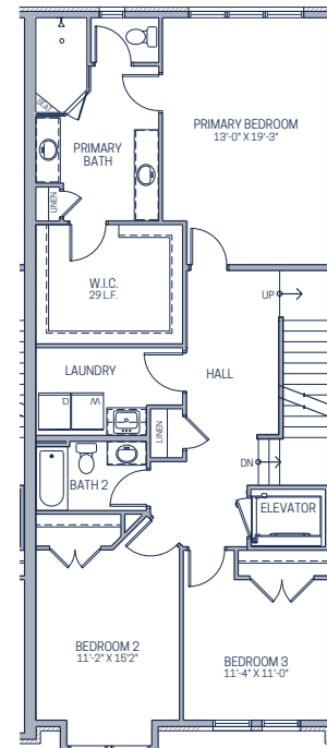
SECOND FLOOR PLAN LOT 109
