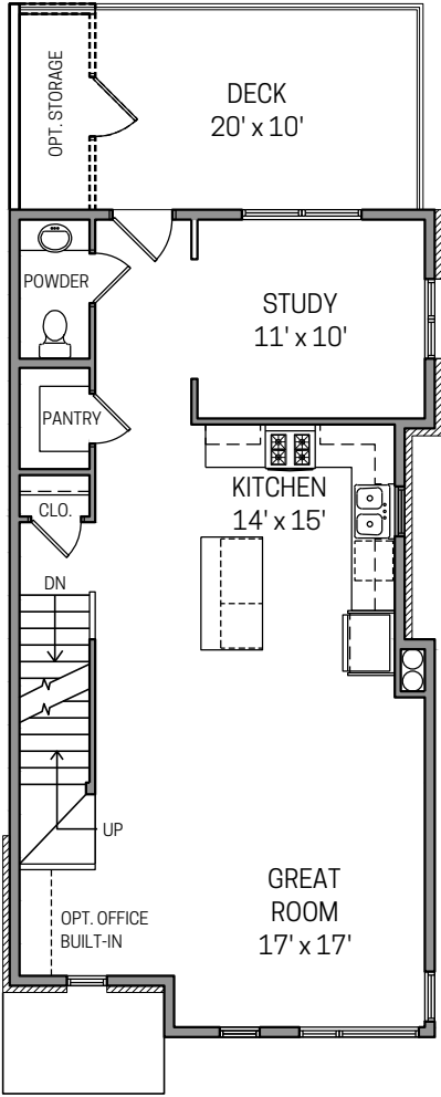
REAR STUDY
