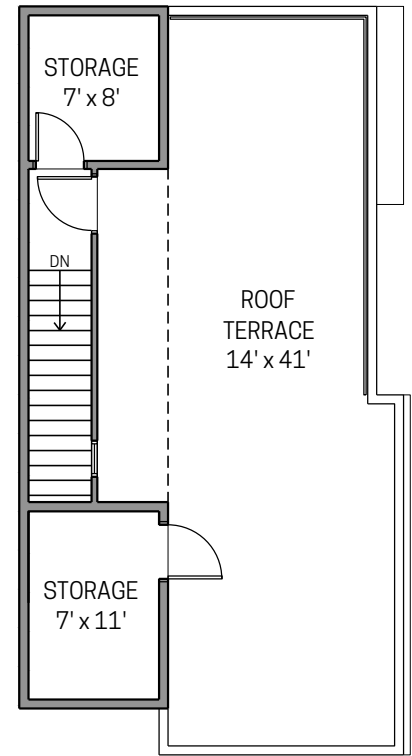
TERRACE
