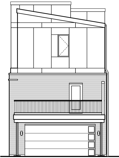
REAR ELEVATION
