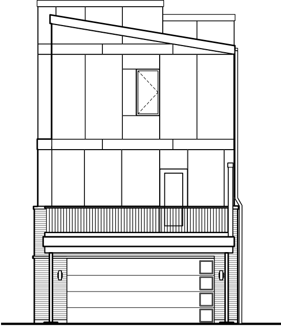
REAR ELEVATION
