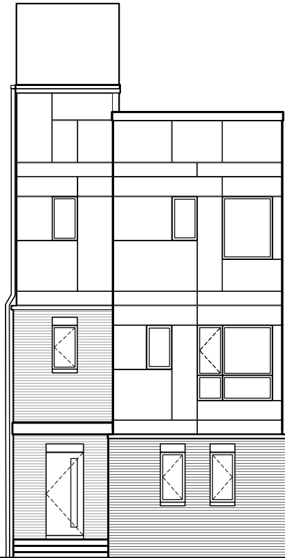
FRONT ELEVATION
