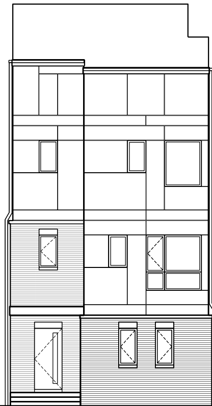
FRONT ELEVATION
