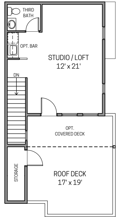
STUDIO / LOFT
