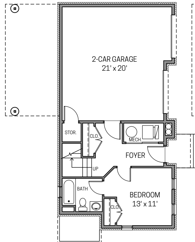
FIRST FLOOR PLAN OPTION
